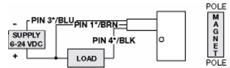
NPN Sinking
