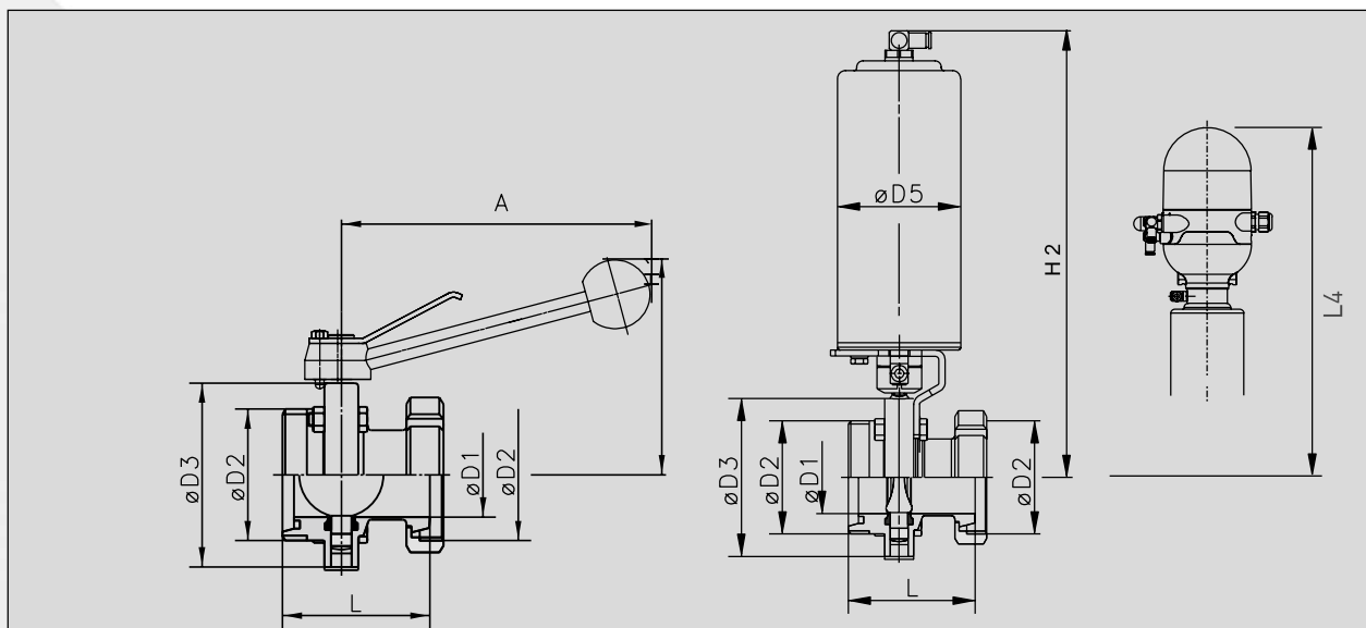
K 581 manually operated Male/slotted nut and liner
