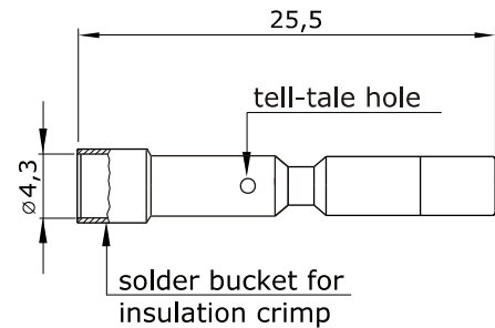
Main Dimensions contact socket
